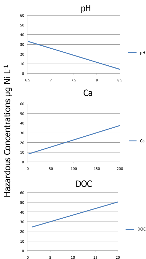
Figure 1.2 Predicted 'stylised' changes in the ecotoxicity of dissolved nickel using the bio-met bioavailability tool. Results are expressed as an HC5, for pH, calcium (Ca mg l -1 ) and dissolved organic carbon (DOC mg l -1 ). Individual parameters were varied while the other two parameters remained constant (pH 7, Ca 120 mg l -1 , DOC 2 mg l -1 ) (from: EC 2010a).
