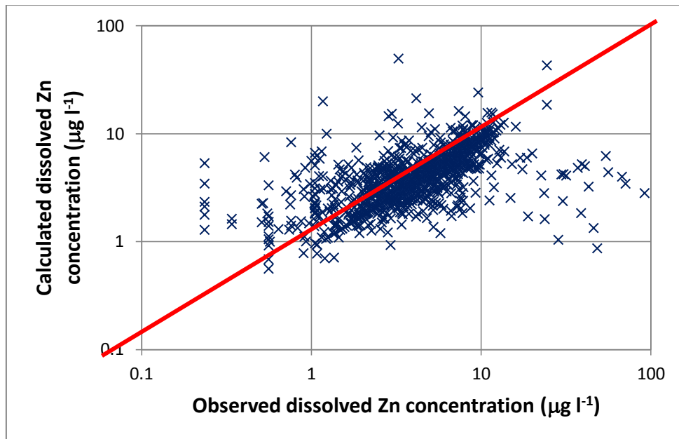
Figure 4.1 Performance of predictions of dissolved Zn from total Zn freshwater data (from Environment Agency 2009e). The line represents the optimal 1:1 agreement.
