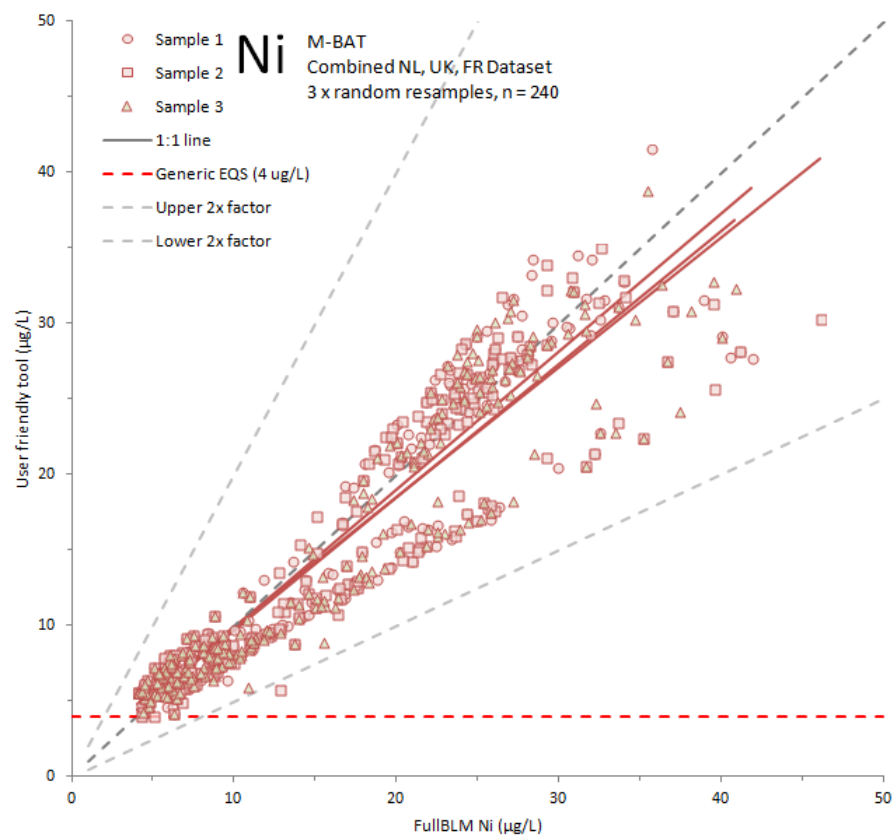
Figure A2.2 Comparison of full BLM predictions for nickel against user-friendly tool predictions for freshwater sites from the Netherlands, France and UK.
