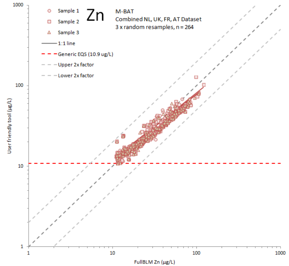
Figure A2.4 Comparison of full BLM predictions for zinc against user-friendly tool predictions for freshwater sites from the Netherlands, France, Austria and UK.
