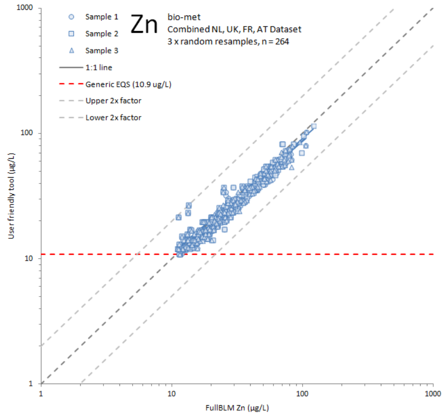
Figure A2.4 Comparison of full BLM predictions for zinc against user-friendly tool predictions for freshwater sites from the Netherlands, France, Austria and UK.
