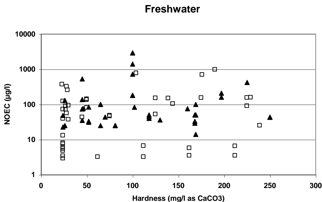
Figure 1.1 Relationship between hardness in freshwater and zinc toxicity, expressed as the NOEC (from: EU 2004).
