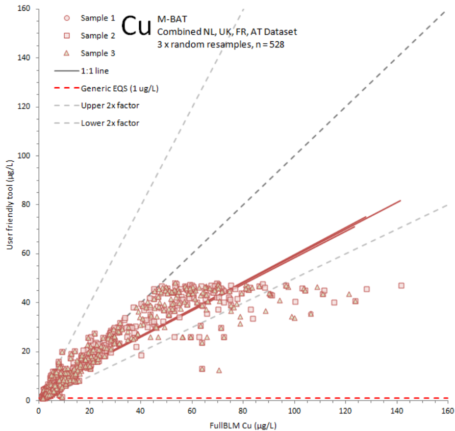
Figure A2.3 Comparison of full BLM predictions for copper against user-friendly tool predictions for freshwater sites from the Netherlands, France, Austria and UK.
