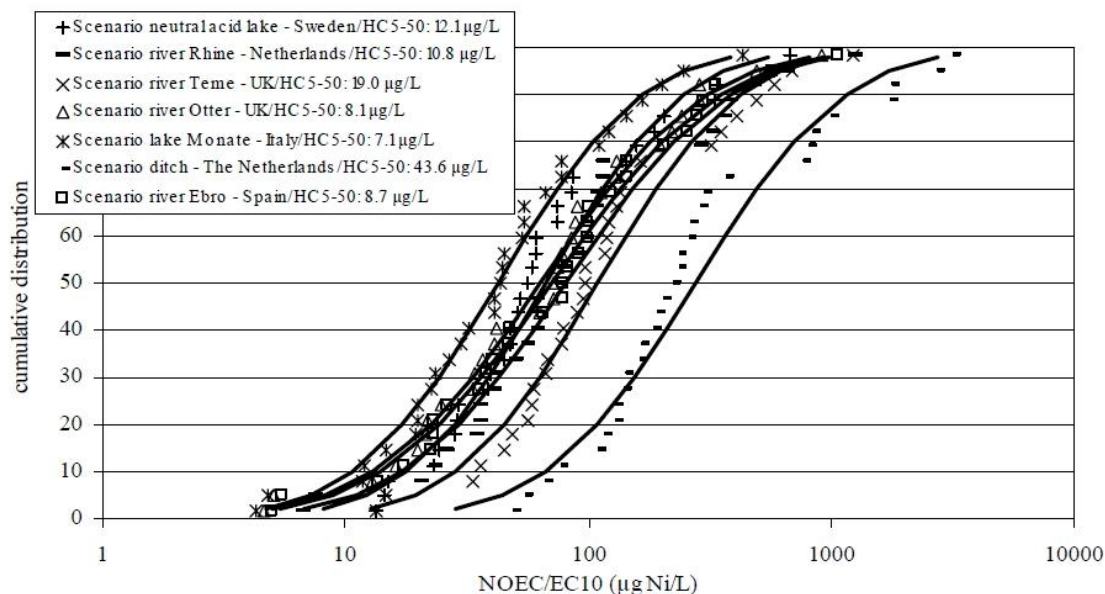
Figure 2.2 Examples of “full normalisation” of nickel SSD based on different water physico-chemistry (from EC 2008).
